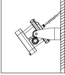
No.3 Wall Mounting
